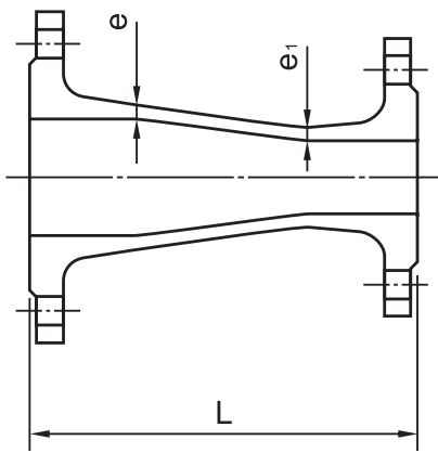
● Concentric Taper
